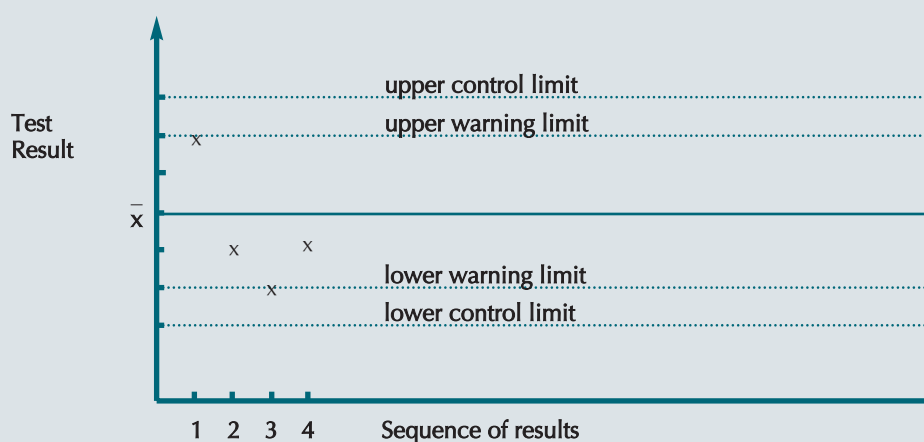
Figure 3 - Example of control chart with breach indicators
