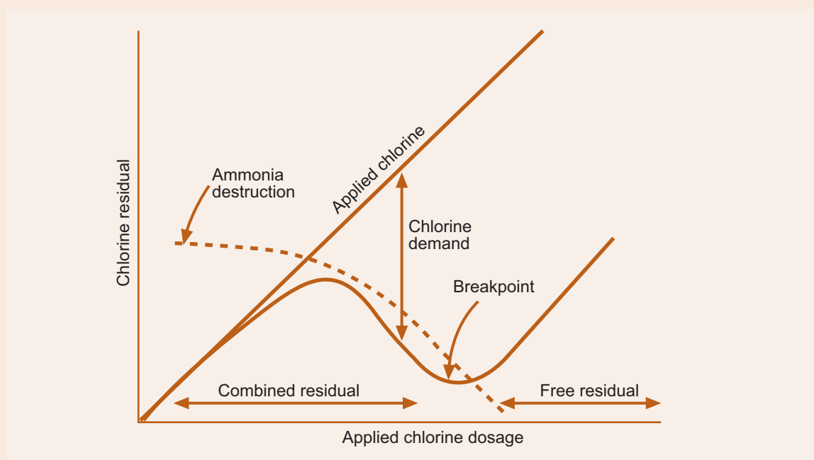
Typical breakpoint chlorination curve
